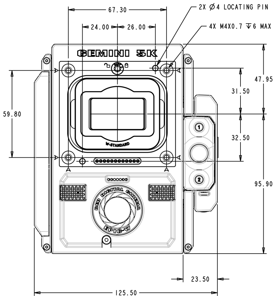
Figure: EPIC-W 5K S35 Front View
