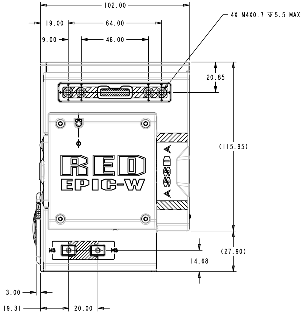
Figure: EPIC-W 5K S35 Side View (Right)
