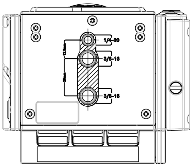
Figure: EPIC-W 5K S35 Bottom View
