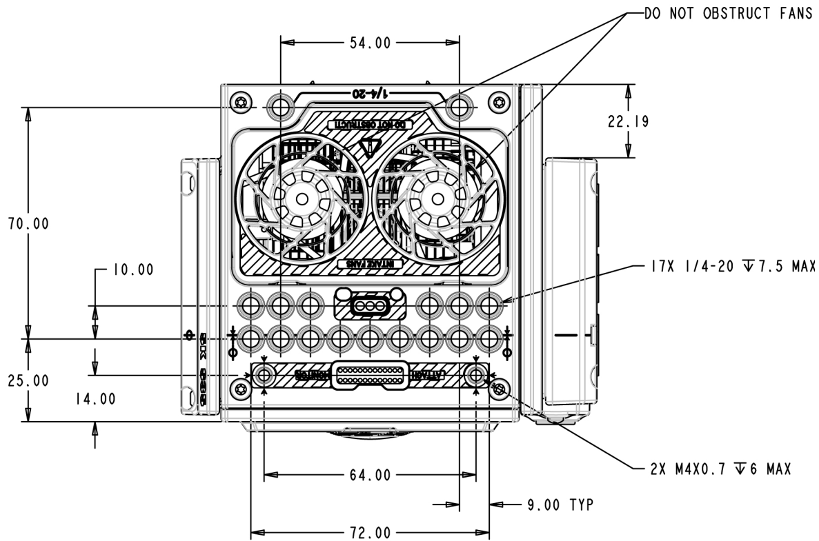
Figure: EPIC-W 5K S35 Top View
