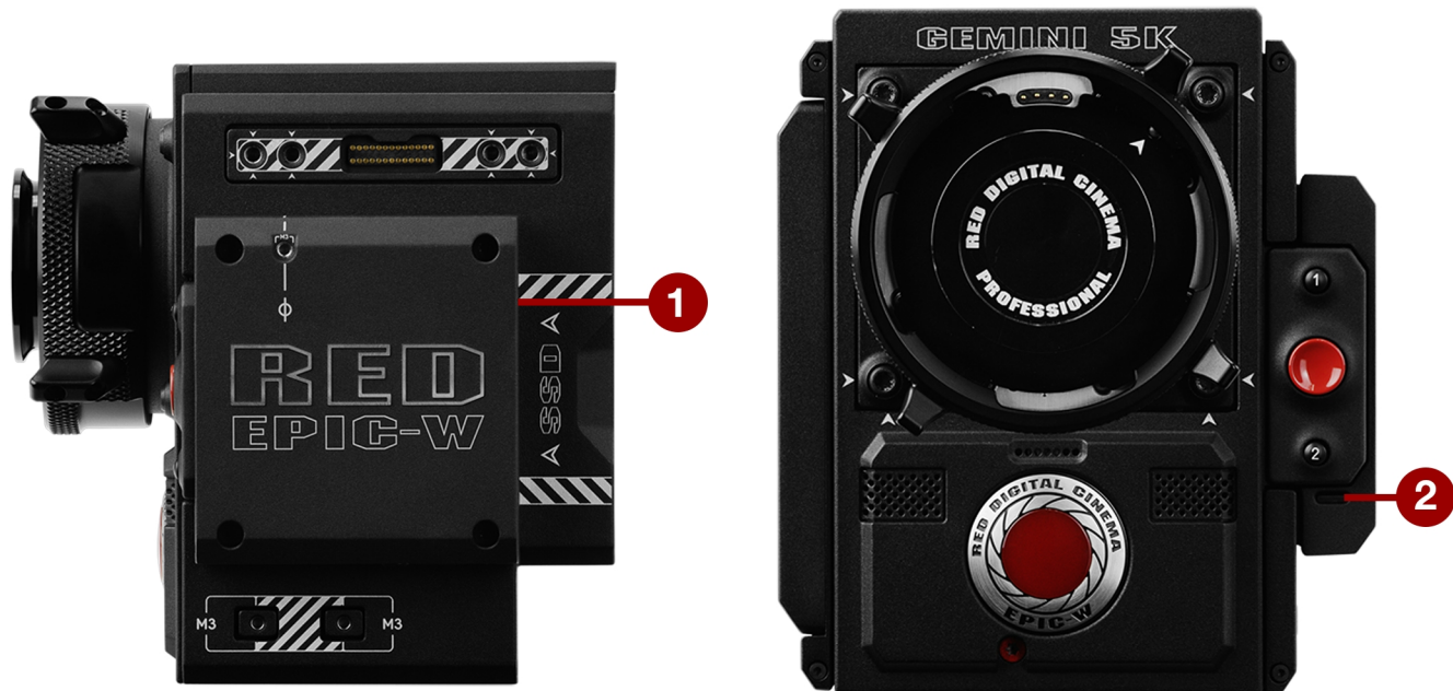
Figure: EPIC-W 5K S35 Media Bay LEDs
