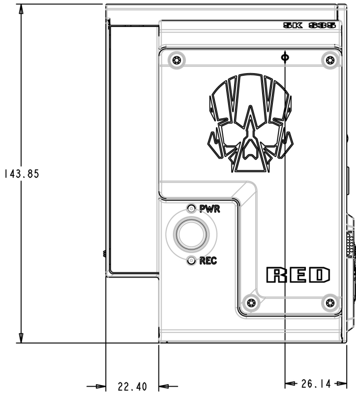
Figure: EPIC-W 5K S35 Side View (Left)
