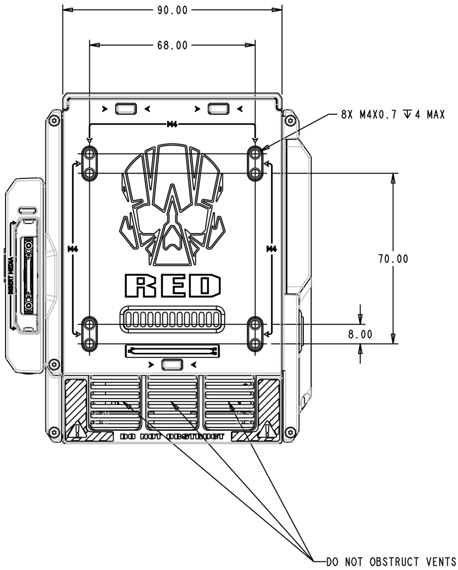
Figure: EPIC-W 5K S35 Back View
