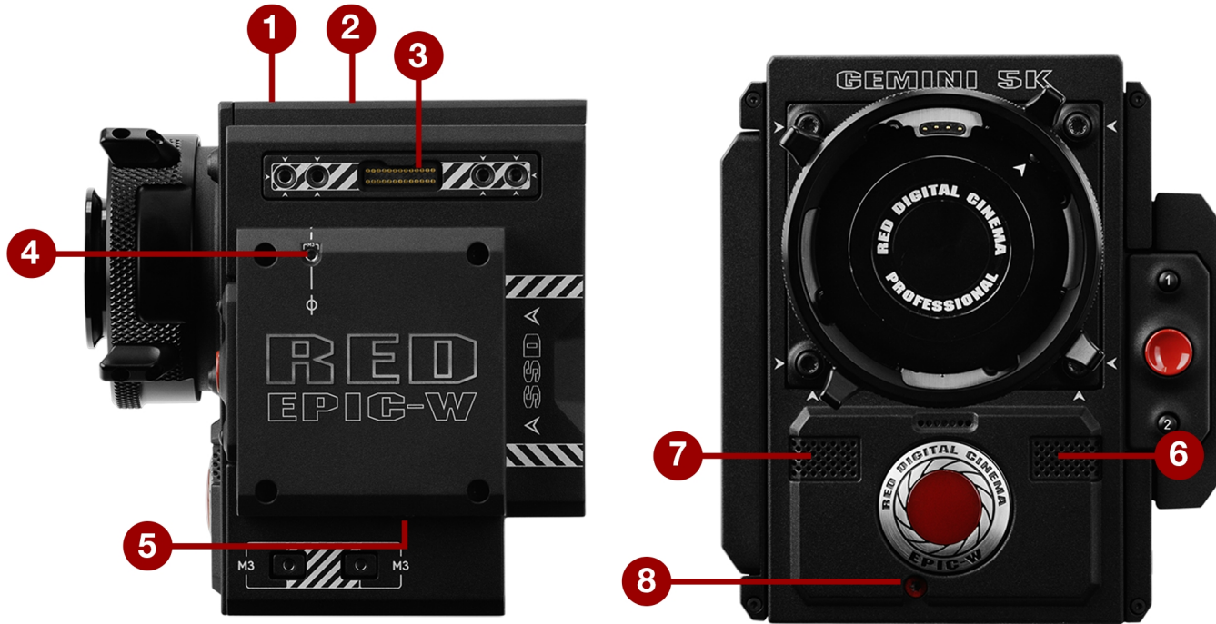
Figure: EPIC-W 5K S35 Ports and Features
